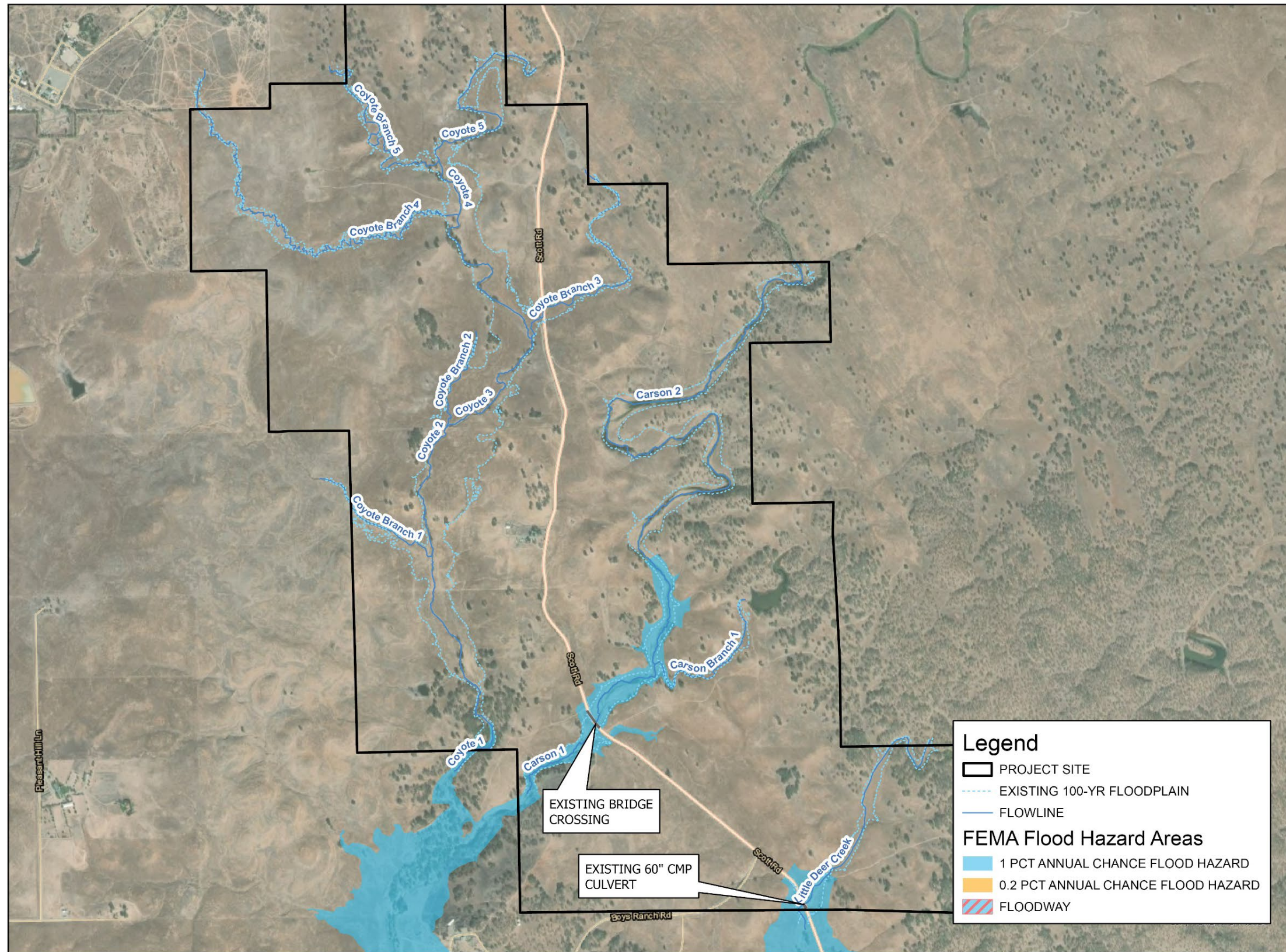
Plate HYD-2: Existing Conditions 100-Year Floodplain
