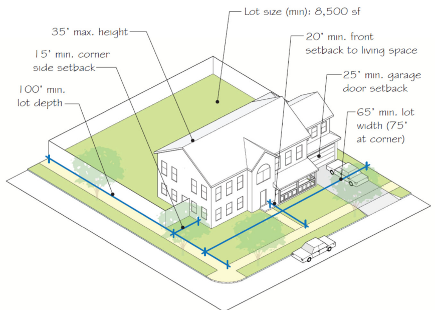
FIGURE 4-2: VLDR DEVELOPMENT PROTOTYPE EXAMPLE
