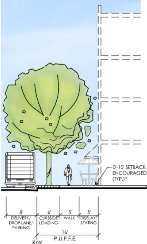
FIGURE 3-5: URBAN SIDEWALK SECTION VIEW
