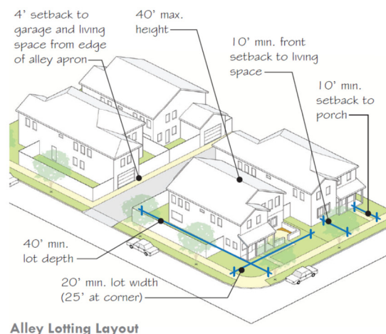
FIGURE 4-5: MDR DEVELOPMENT PROTOTYPE EXAMPLES
